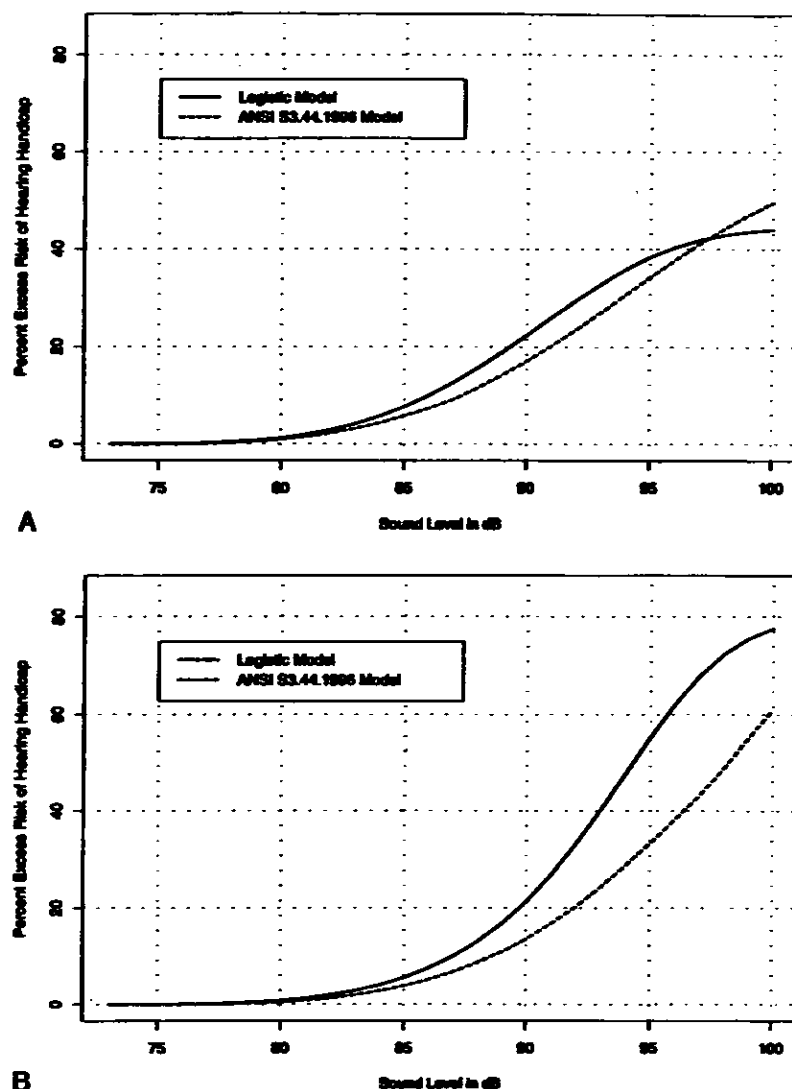
FIG. 5. Excess risk (A1-weighting, 1–4 kHz) as a function of sound level ( L_{\text{Aeq}} ) according to model 4 (Table IV), in comparison with curves derived from ANSI S3.44.1996 using Annex A database. Panel A: age 65 years, exposure duration 45 years. Panel B: age 45 years, exposure duration 25 years.
