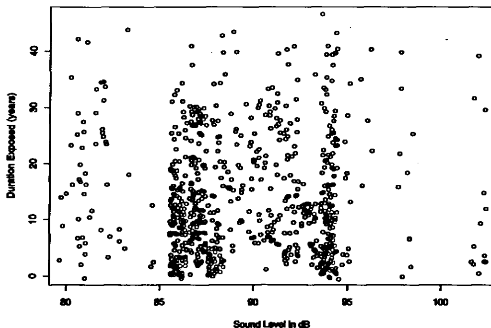
FIG. 2. Scatter plot of exposure sound levels ( L_{AE} ) versus exposure duration of 792 noise-exposed workers from the NIOSH 1968-72 survey.
